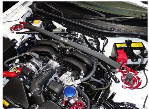
Toyota GR86 ZN8 Front Installation Example
