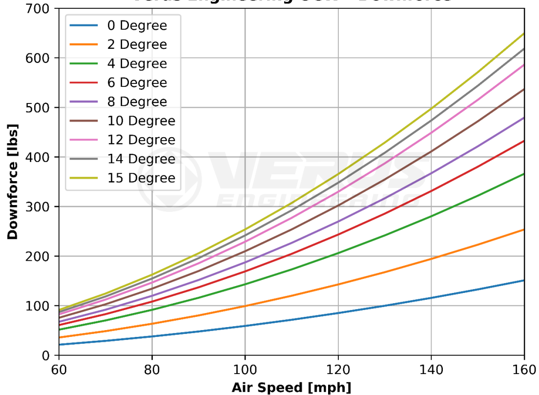
Verus Engineering UCW - Downforce
