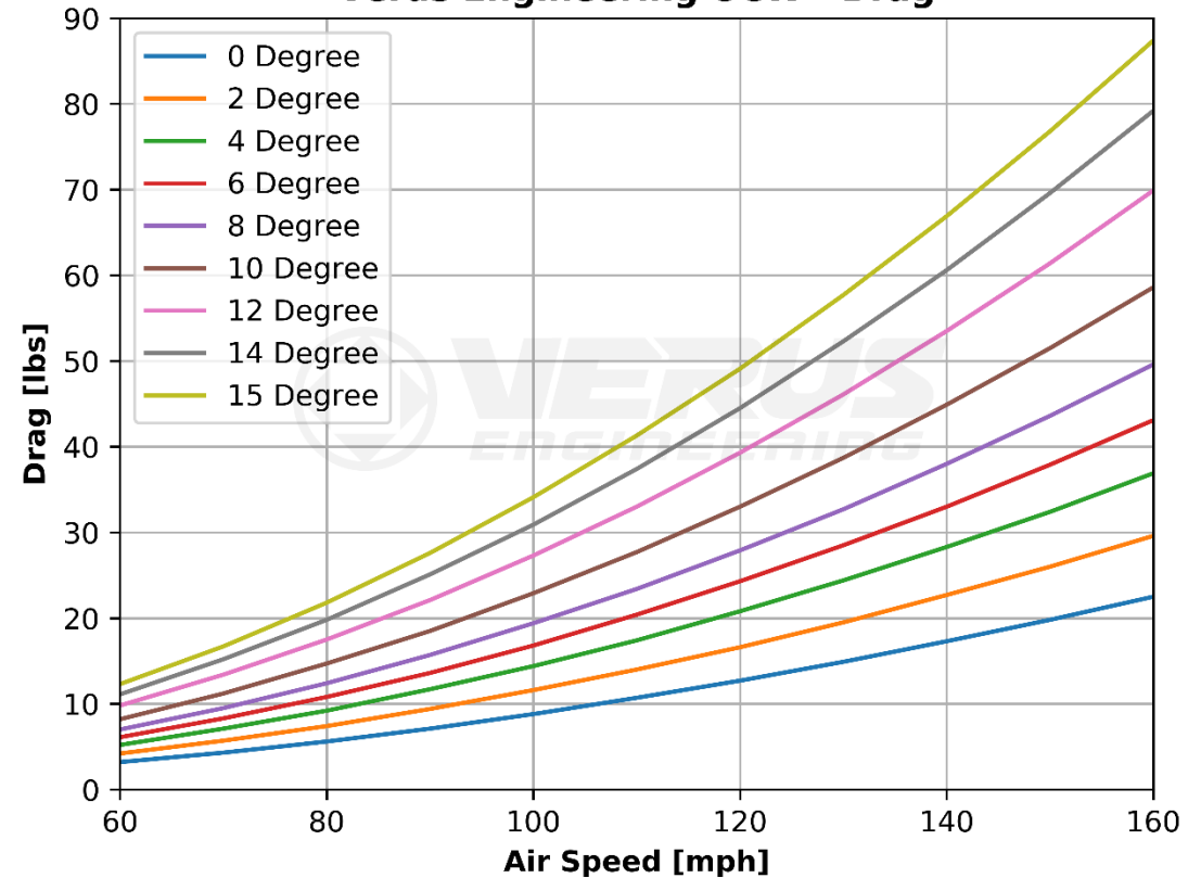
Verus Engineering UCW - Drag
