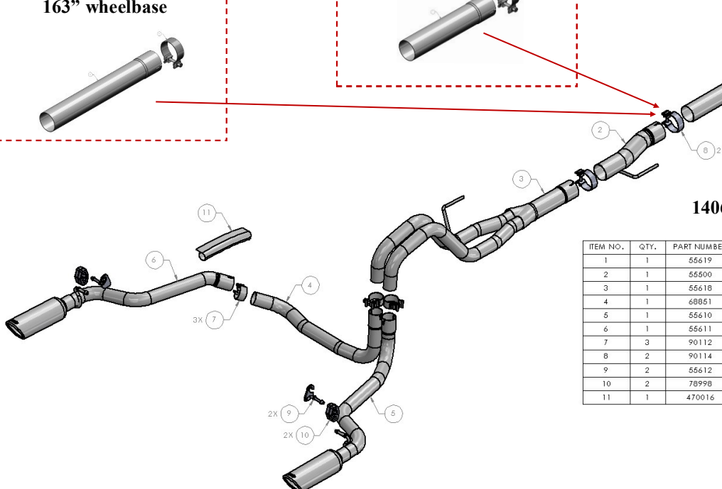
(PN-60564) ADAPTOR 163" wheelbase
